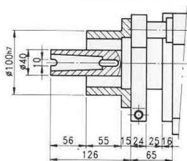
FD75M-100-MT3A Multi
