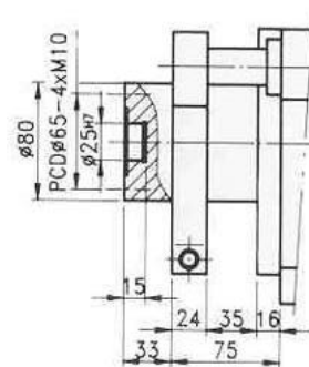
FD75-100-FB30
