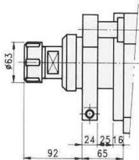
FD75M-100-MT3A Multi
